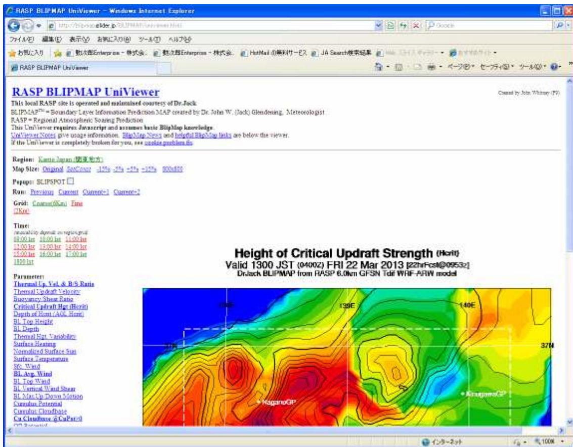
図2 UniViewer
