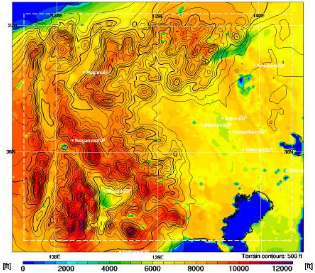
図5 Height of Critical Updraft Strength ( H_{crit} )の例
